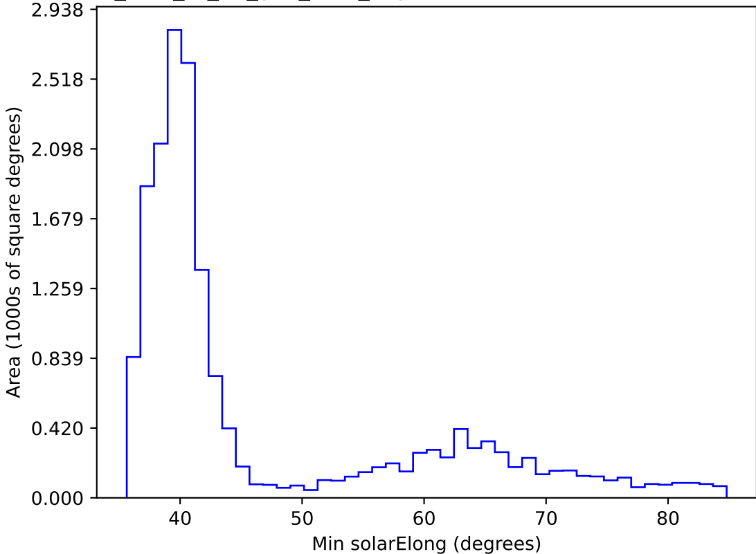
too_elab_r8_d2_griz_v3.4_10yrs WFD all bands: Min solarElong
