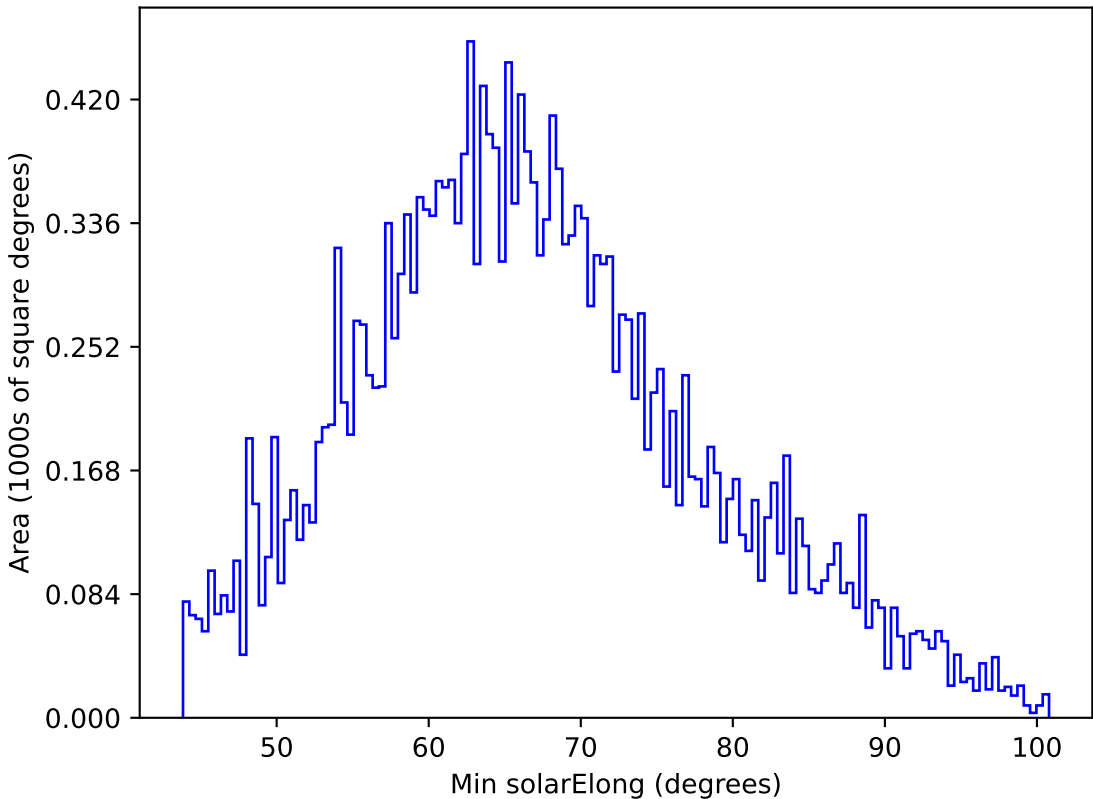
too_elab_r8_d2_griz_v3.4_10yrs All sky y band: Min solarElong
