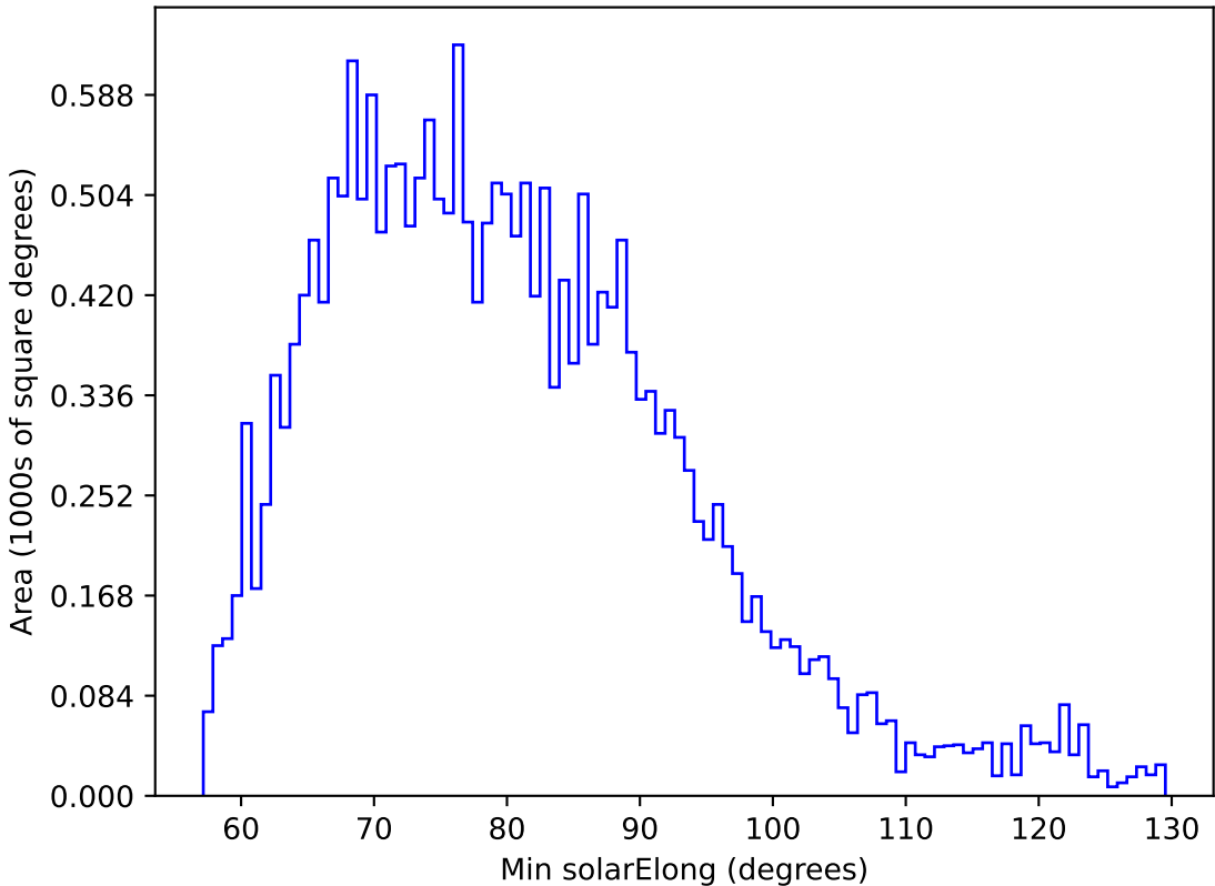
too_elab_r8_d2_griz_v3.4_10yrs All sky u band: Min solarElong
