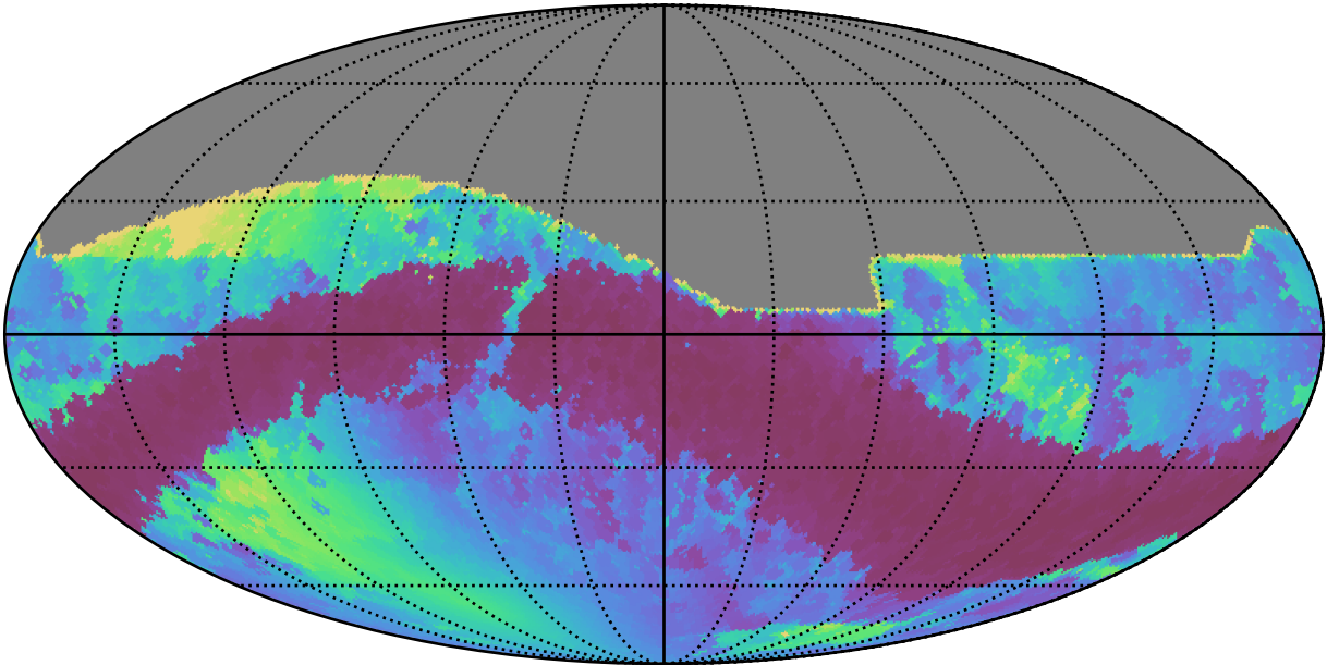
too_elab_r8_d2_griz_v3.4_10yrs All sky r band: Min solarElong
