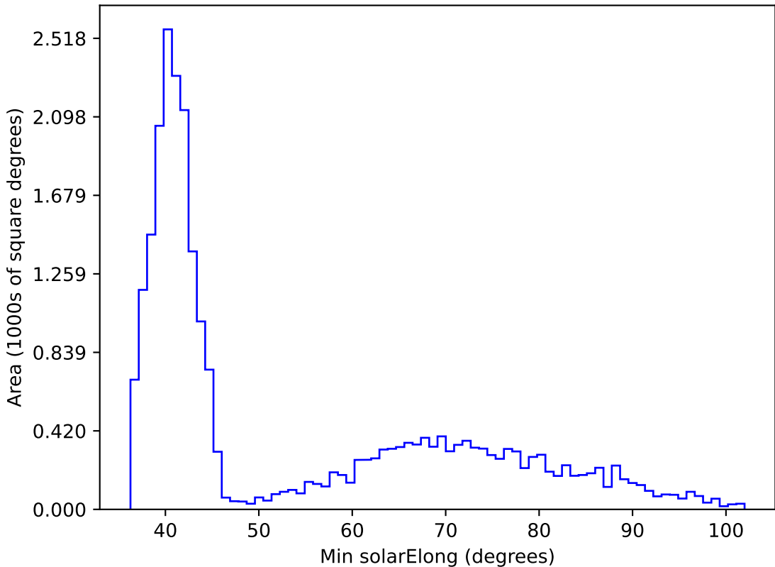
too_elab_r8_d2_griz_v3.4_10yrs All sky i band: Min solarElong
