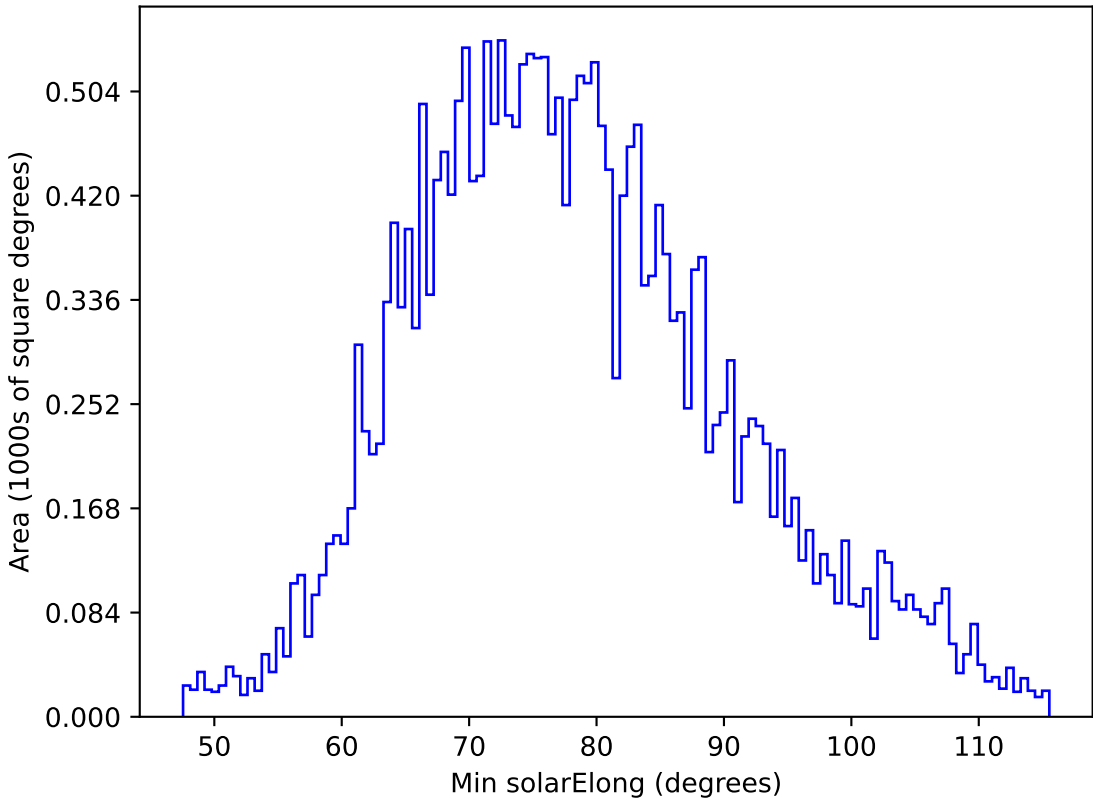
too_elab_r8_d2_griz_v3.4_10yrs All sky g band: Min solarElong
