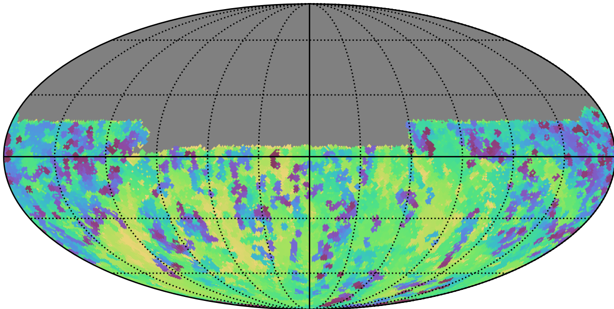
too_elab_r8_d2_griz_v3.4_10yrs Yr 1 y band: Min skyBrightness
