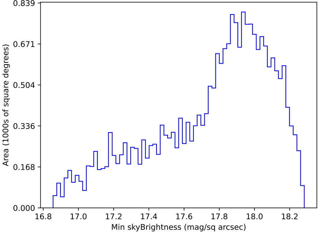
too_elab_r8_d2_griz_v3.4_10yrs Yr 1 y band: Min skyBrightness
