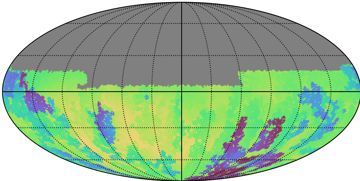
too_elab_r8_d2_griz_v3.4_10yrs Yr 1 u band: Min skyBrightness
