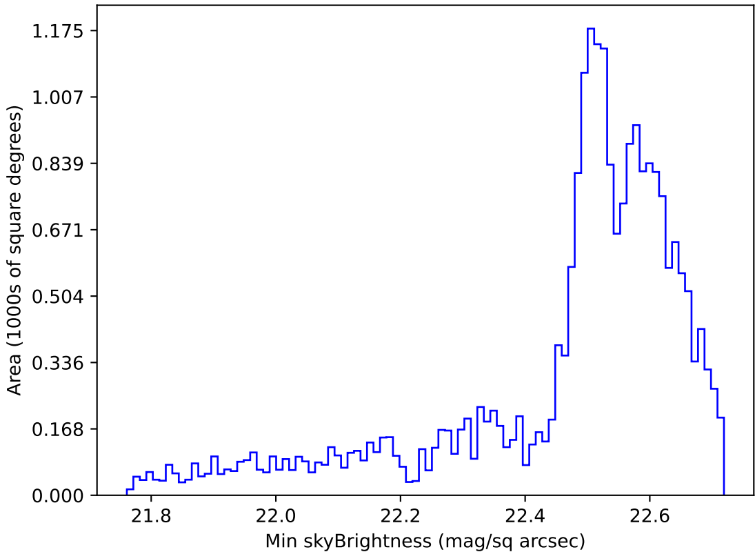
too_elab_r8_d2_griz_v3.4_10yrs Yr 1 u band: Min skyBrightness
