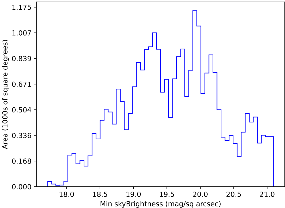
too_elab_r8_d2_griz_v3.4_10yrs Yr 1 r band: Min skyBrightness
