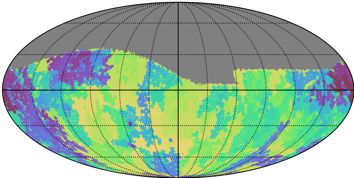
too_elab_r8_d2_griz_v3.4_10yrs Yr 1 g band: Min skyBrightness
