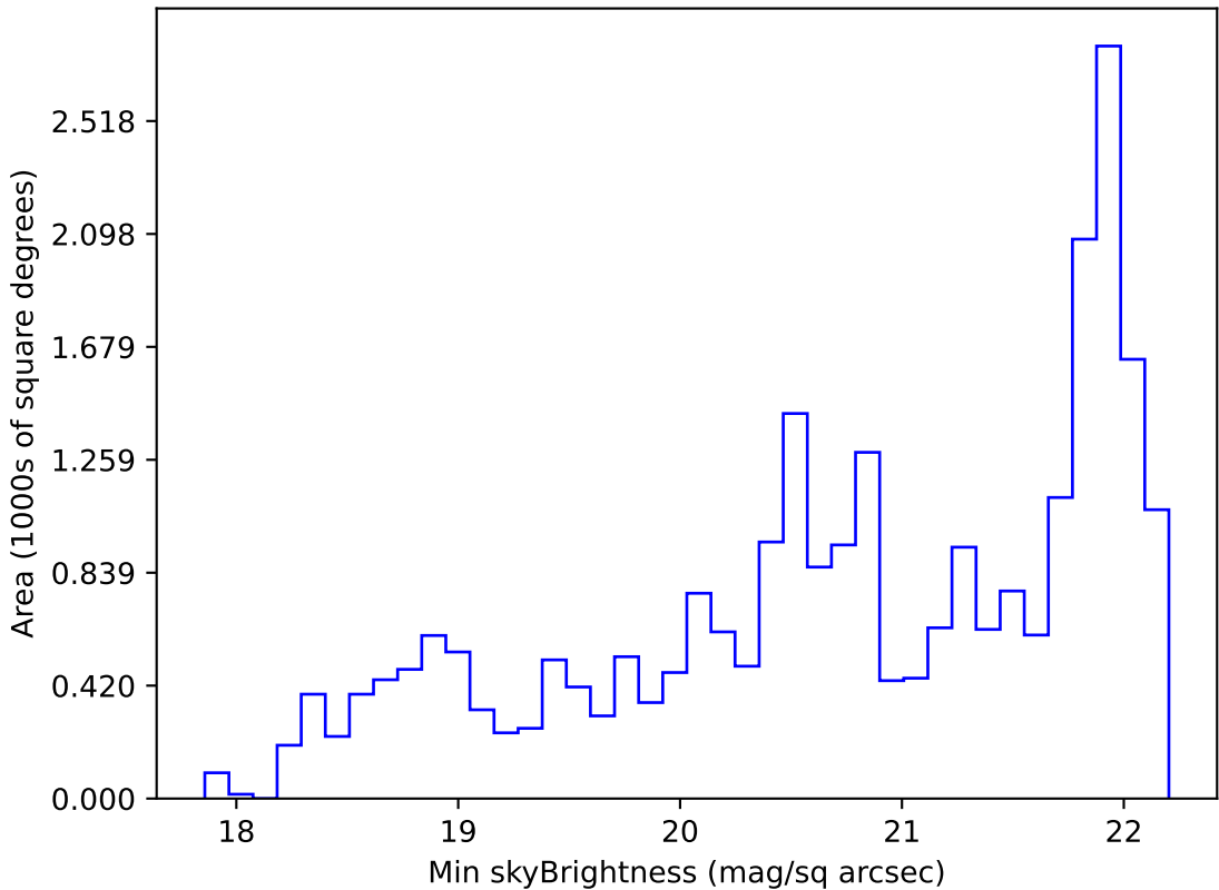
too_elab_r8_d2_griz_v3.4_10yrs Yr 1 g band: Min skyBrightness
