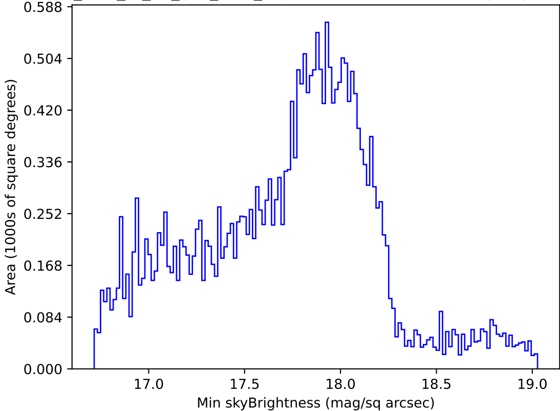
too_elab_r8_d2_griz_v3.4_10yrs Yr 1 all bands: Min skyBrightness
