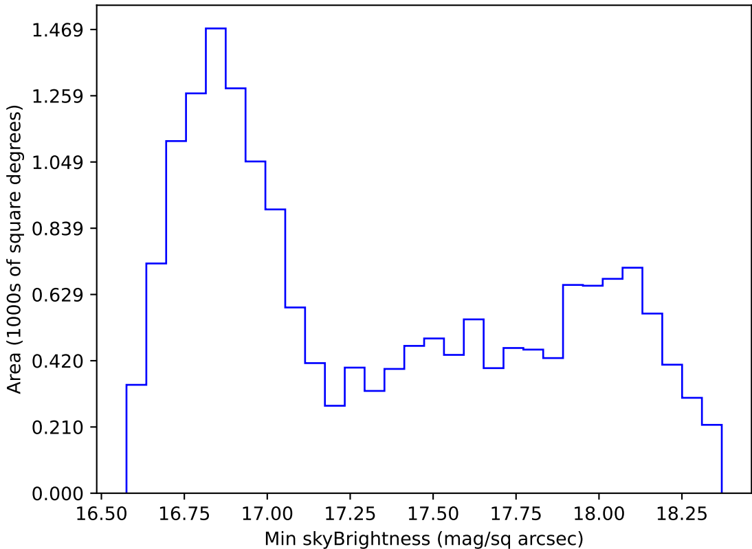
too_elab_r8_d2_griz_v3.4_10yrs WFD z band: Min skyBrightness
