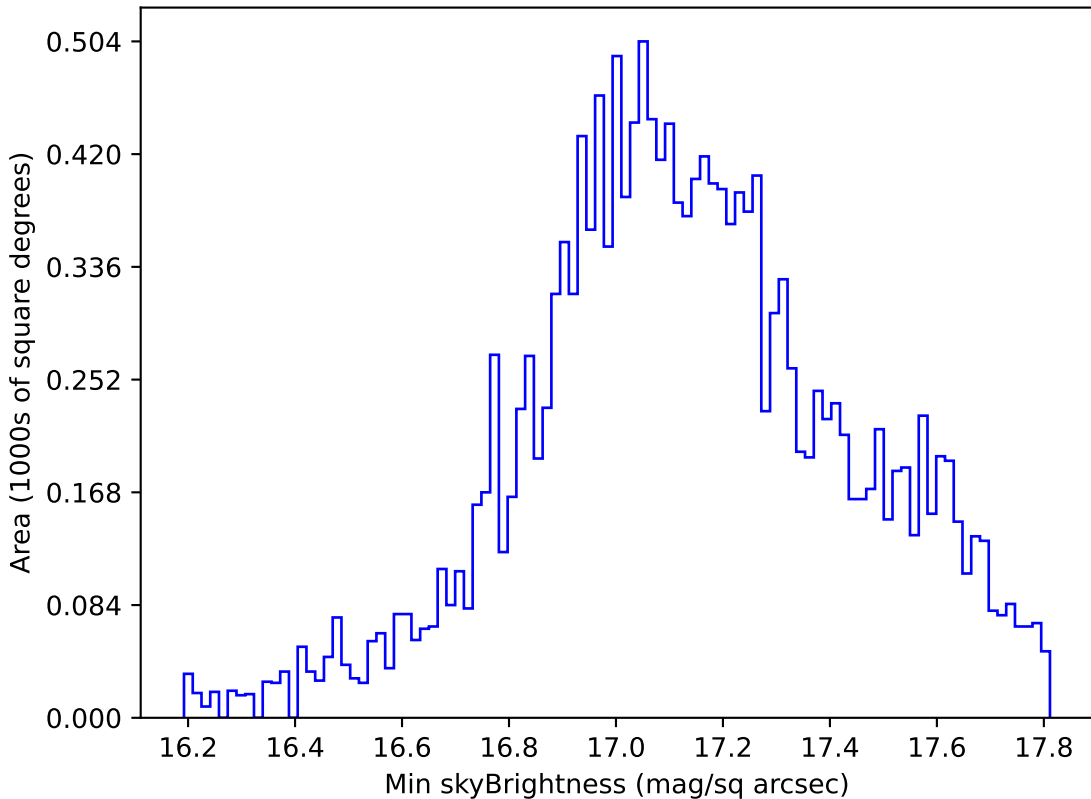
too_elab_r8_d2_griz_v3.4_10yrs WFD y band: Min skyBrightness
