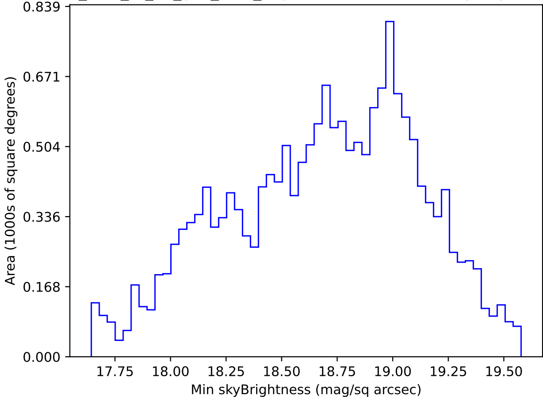
too_elab_r8_d2_griz_v3.4_10yrs WFD r band: Min skyBrightness
