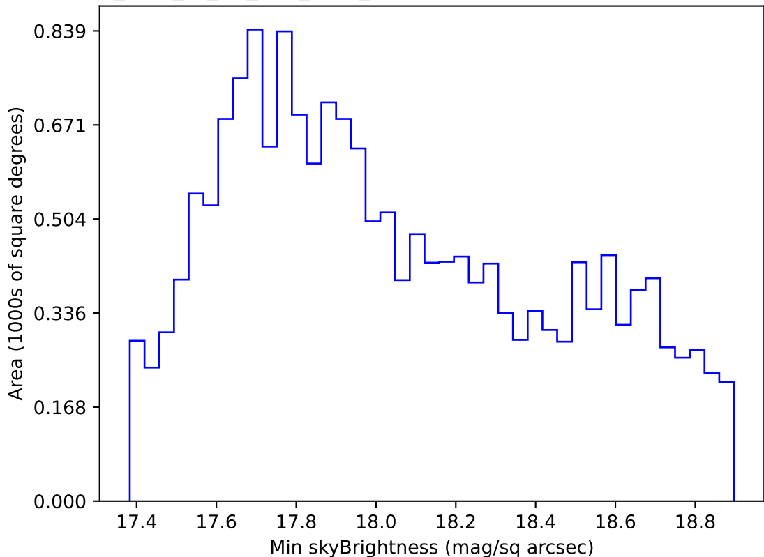
too_elab_r8_d2_griz_v3.4_10yrs WFD i band: Min skyBrightness
