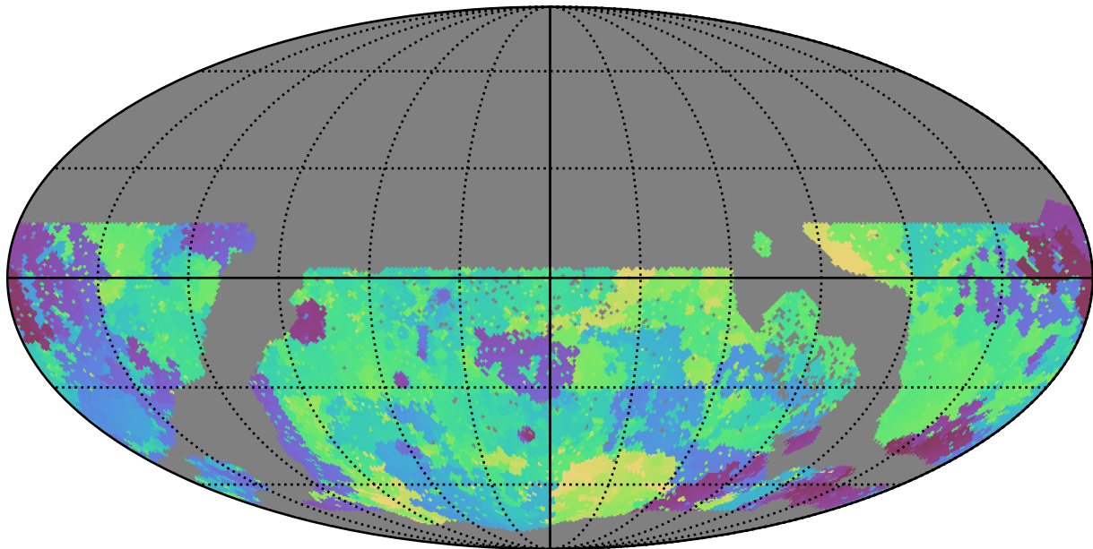
too_elab_r8_d2_griz_v3.4_10yrs WFD g band: Min skyBrightness
