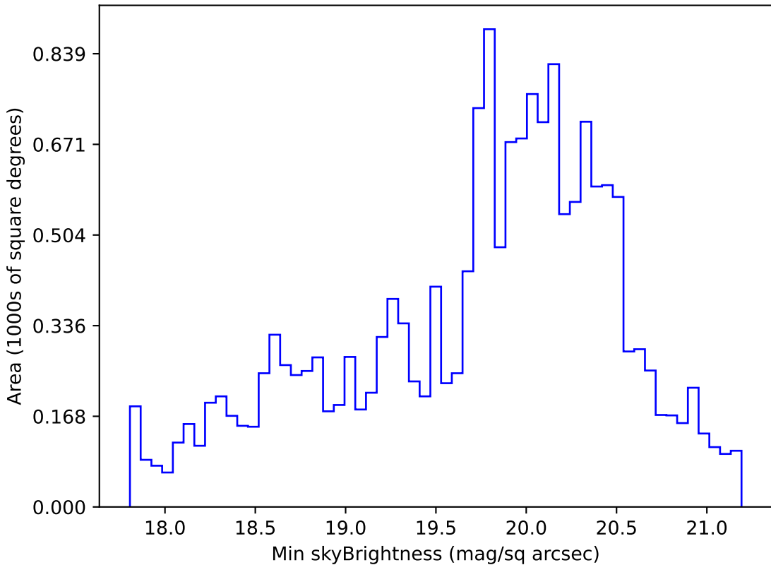
too_elab_r8_d2_griz_v3.4_10yrs WFD g band: Min skyBrightness
