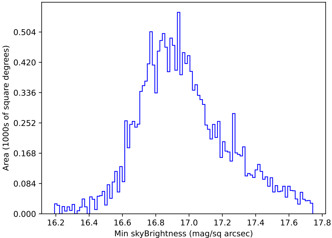
too_elab_r8_d2_griz_v3.4_10yrs WFD all bands: Min skyBrightness
