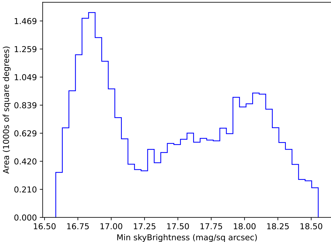
too_elab_r8_d2_griz_v3.4_10yrs All sky z band: Min skyBrightness
