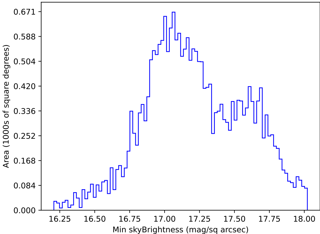
too_elab_r8_d2_griz_v3.4_10yrs All sky y band: Min skyBrightness
