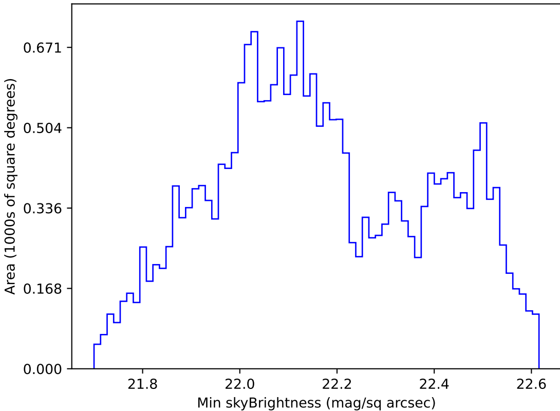
too_elab_r8_d2_griz_v3.4_10yrs All sky u band: Min skyBrightness
