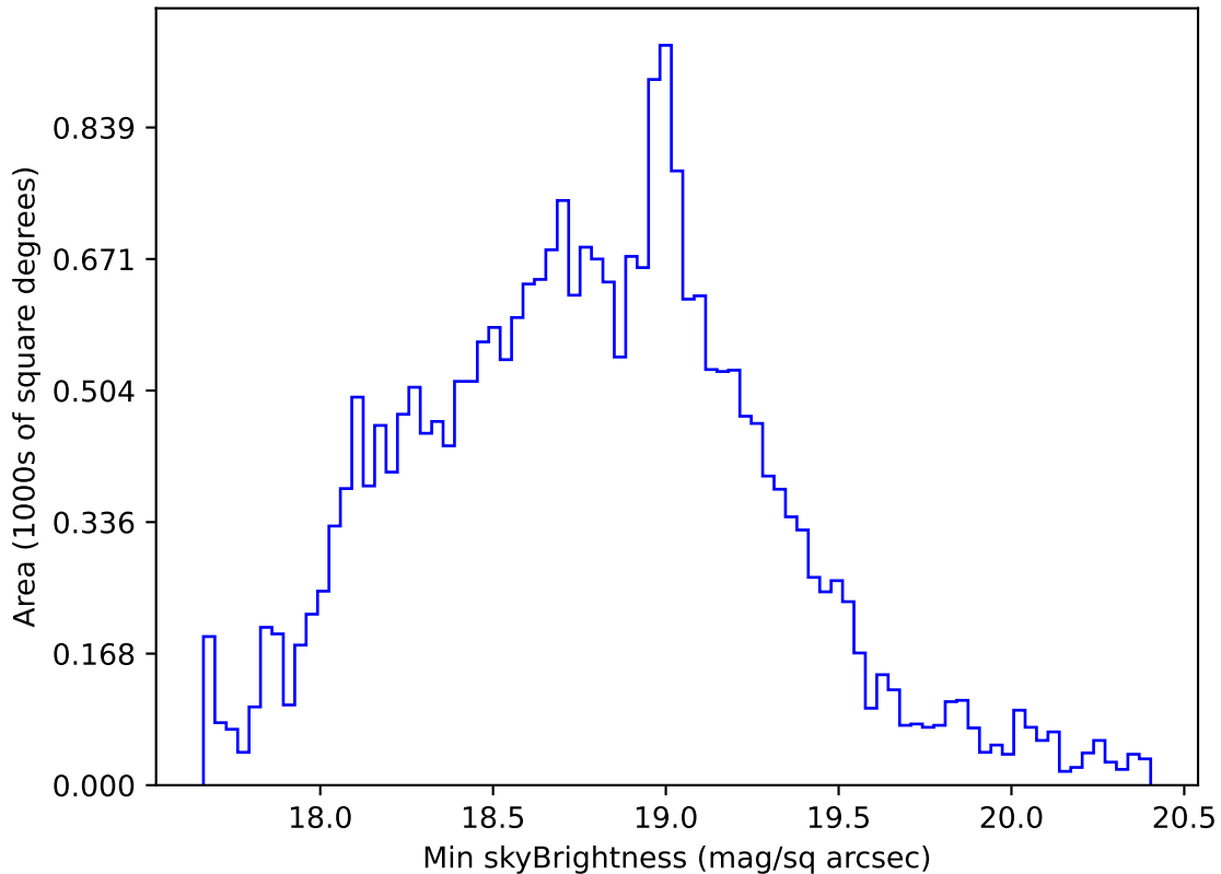
too_elab_r8_d2_griz_v3.4_10yrs All sky r band: Min skyBrightness
