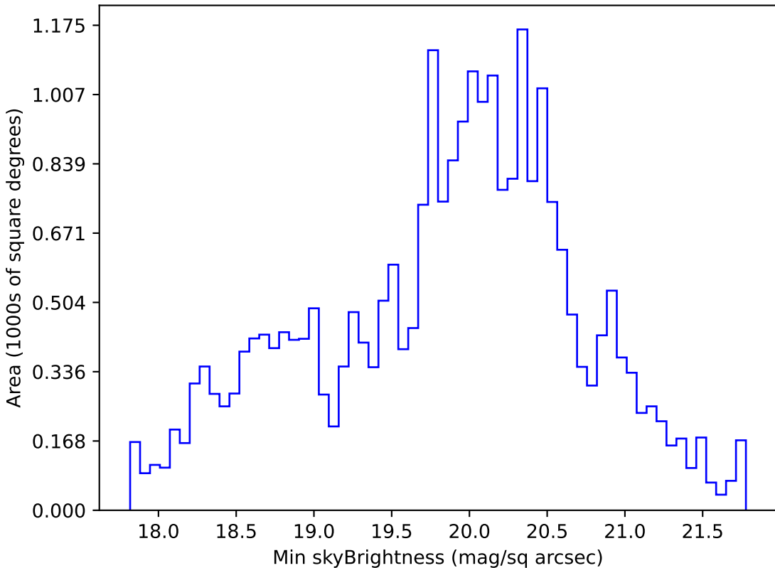
too_elab_r8_d2_griz_v3.4_10yrs All sky g band: Min skyBrightness
