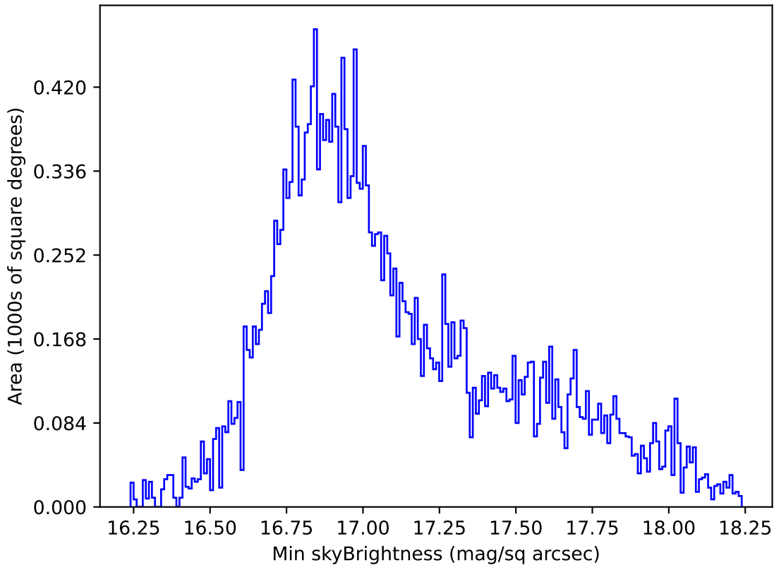
too_elab_r8_d2_griz_v3.4_10yrs All sky all bands: Min skyBrightness
