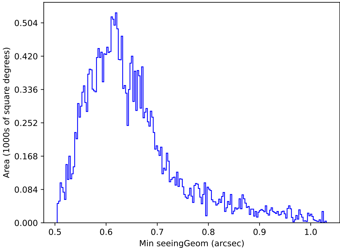
too_elab_r8_d2_griz_v3.4_10yrs Yr 1 z band: Min seeingGeom
