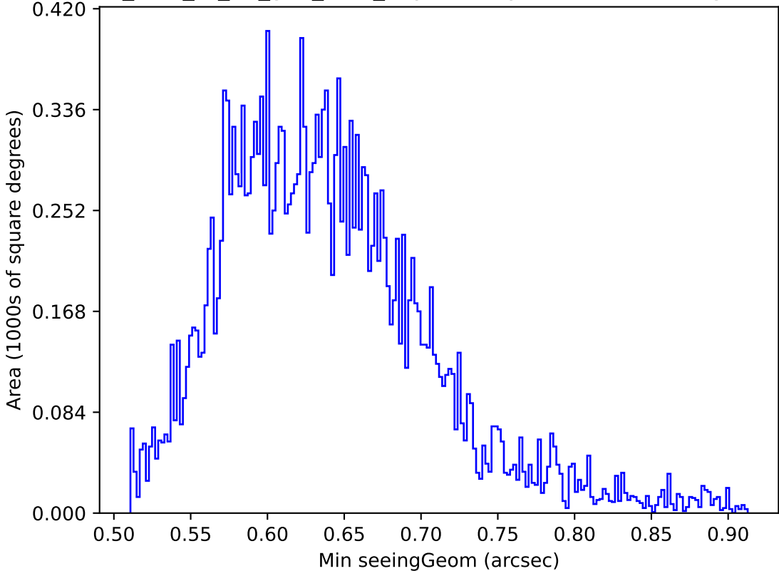
too_elab_r8_d2_griz_v3.4_10yrs Yr 1 y band: Min seeingGeom
