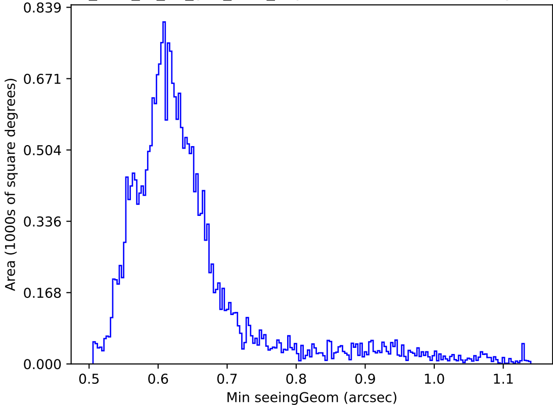
too_elab_r8_d2_griz_v3.4_10yrs Yr 1 r band: Min seeingGeom
