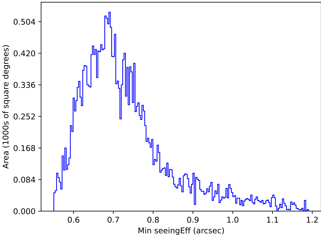
too_elab_r8_d2_griz_v3.4_10yrs Yr 1 z band: Min seeingEff
