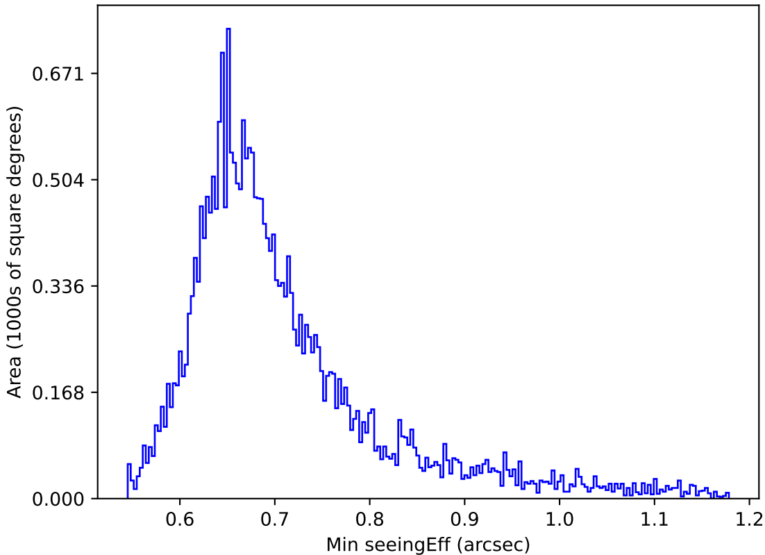
too_elab_r8_d2_griz_v3.4_10yrs Yr 1 i band: Min seeingEff
