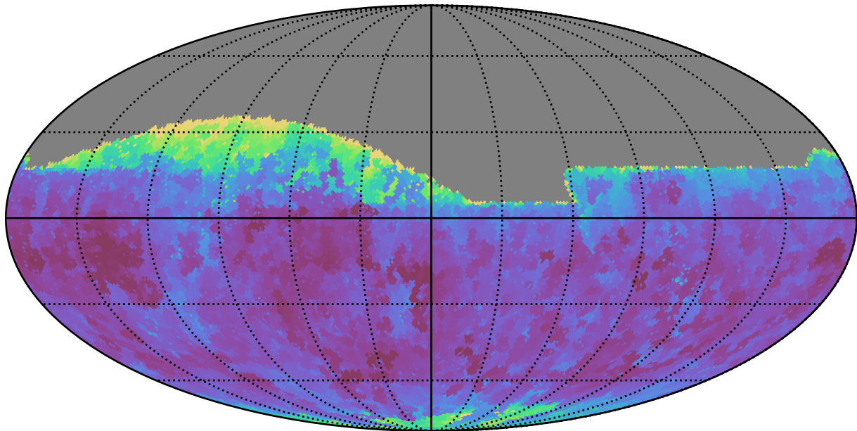
too_elab_r8_d2_griz_v3.4_10yrs Yr 1 all bands: Min seeingEff
