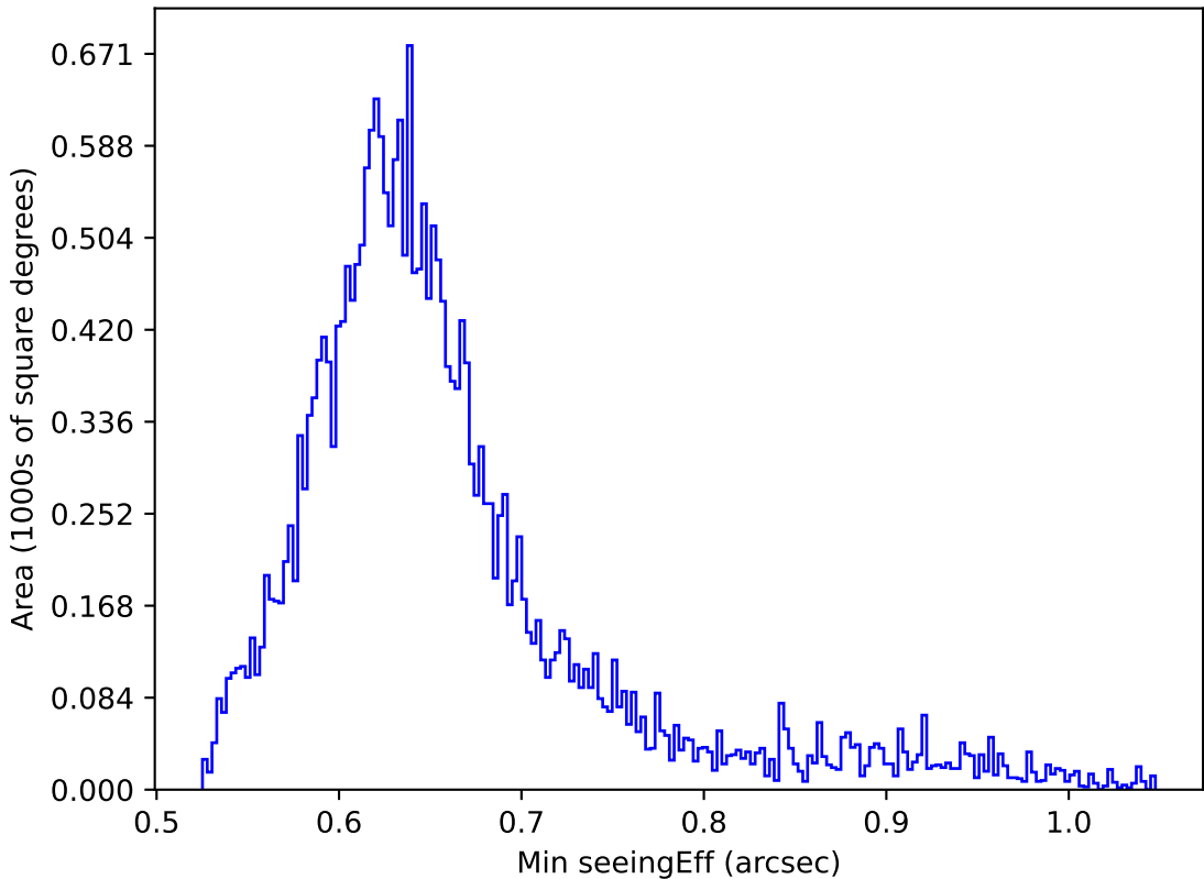
too_elab_r8_d2_griz_v3.4_10yrs Yr 1 all bands: Min seeingEff
