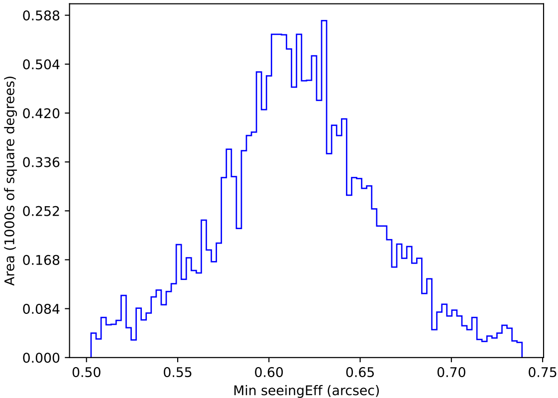
too_elab_r8_d2_griz_v3.4_10yrs WFD z band: Min seeingEff
