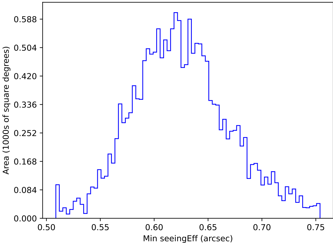
too_elab_r8_d2_griz_v3.4_10yrs WFD y band: Min seeingEff
