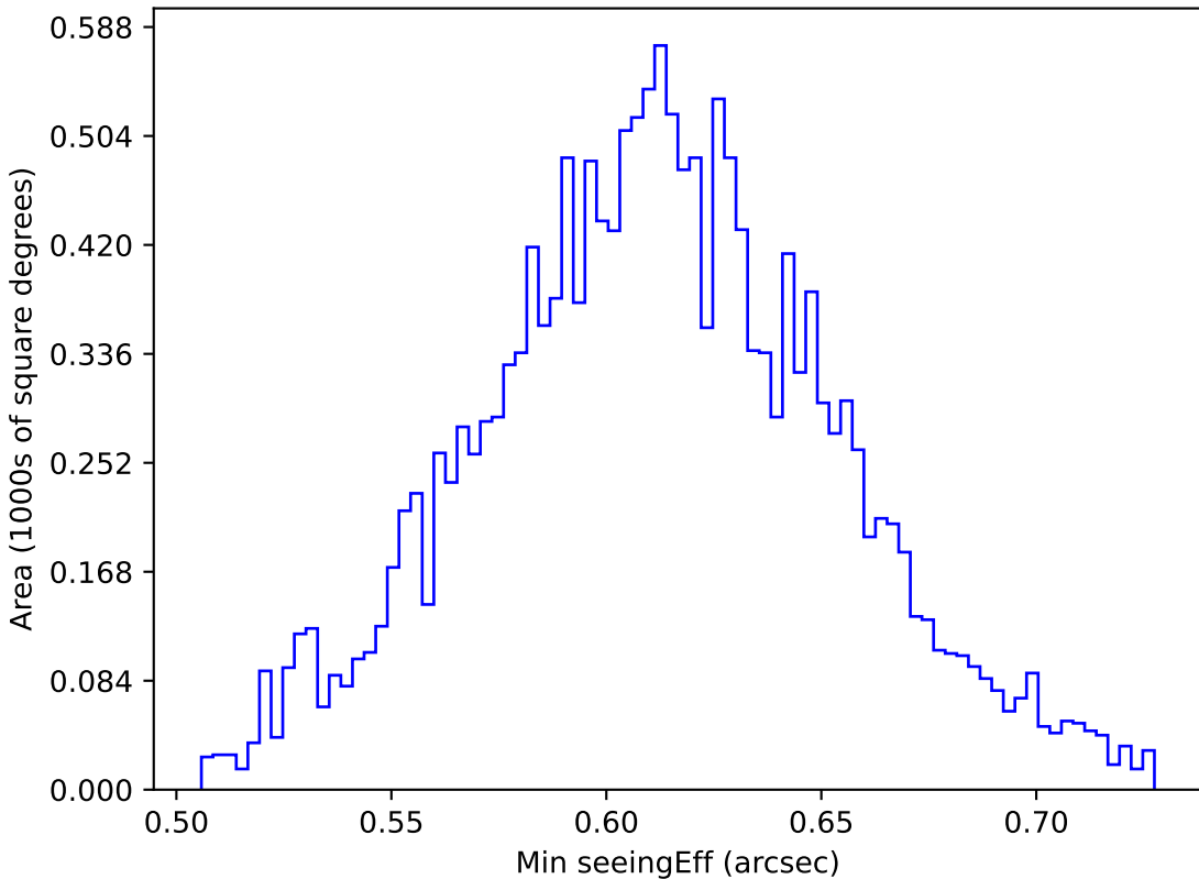
too_elab_r8_d2_griz_v3.4_10yrs WFD r band: Min seeingEff
