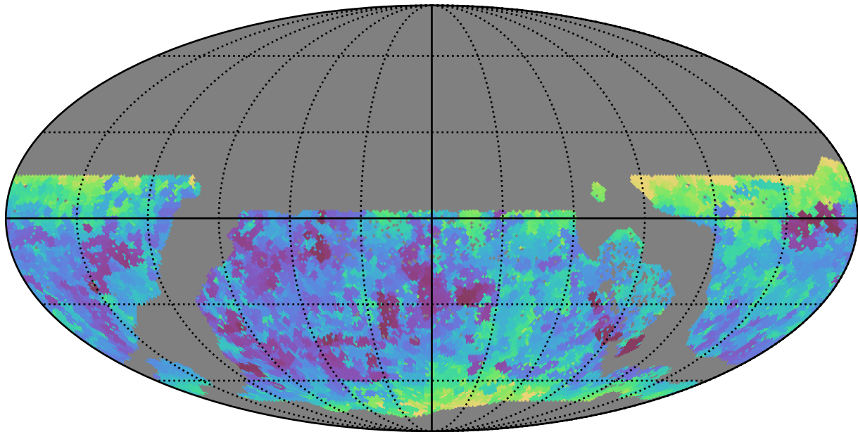
too_elab_r8_d2_griz_v3.4_10yrs WFD i band: Min seeingEff
