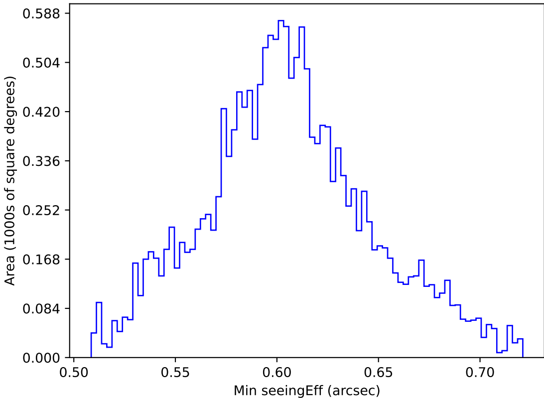
too_elab_r8_d2_griz_v3.4_10yrs WFD i band: Min seeingEff
