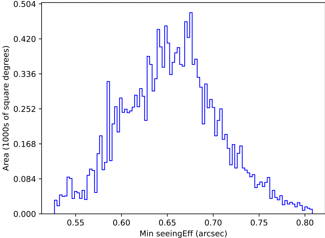
too_elab_r8_d2_griz_v3.4_10yrs WFD g band: Min seeingEff
