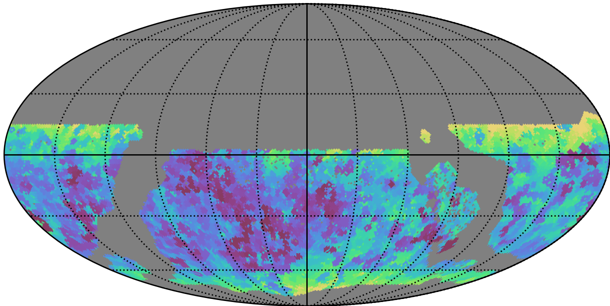
too_elab_r8_d2_griz_v3.4_10yrs WFD all bands: Min seeingEff
