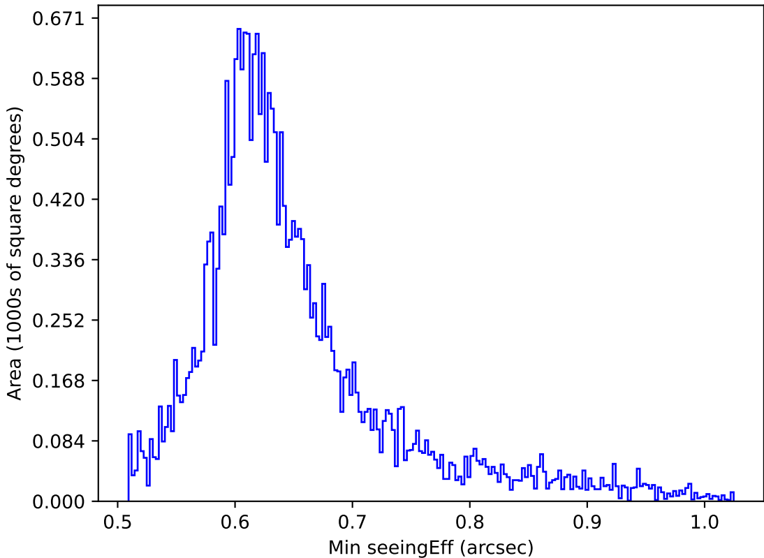
too_elab_r8_d2_griz_v3.4_10yrs All sky z band: Min seeingEff
