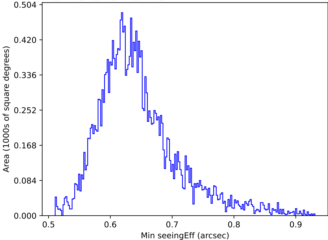
too_elab_r8_d2_griz_v3.4_10yrs All sky y band: Min seeingEff
