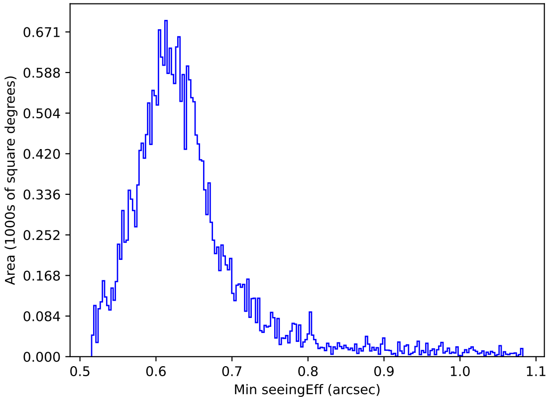
too_elab_r8_d2_griz_v3.4_10yrs All sky r band: Min seeingEff
