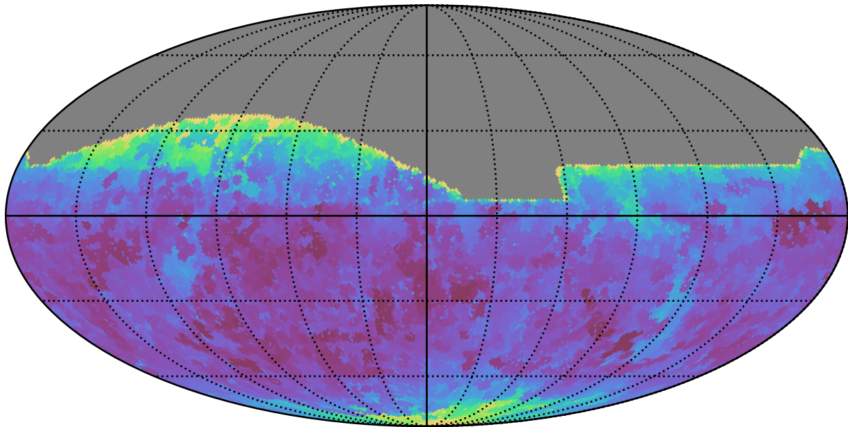
too_elab_r8_d2_griz_v3.4_10yrs All sky i band: Min seeingEff
