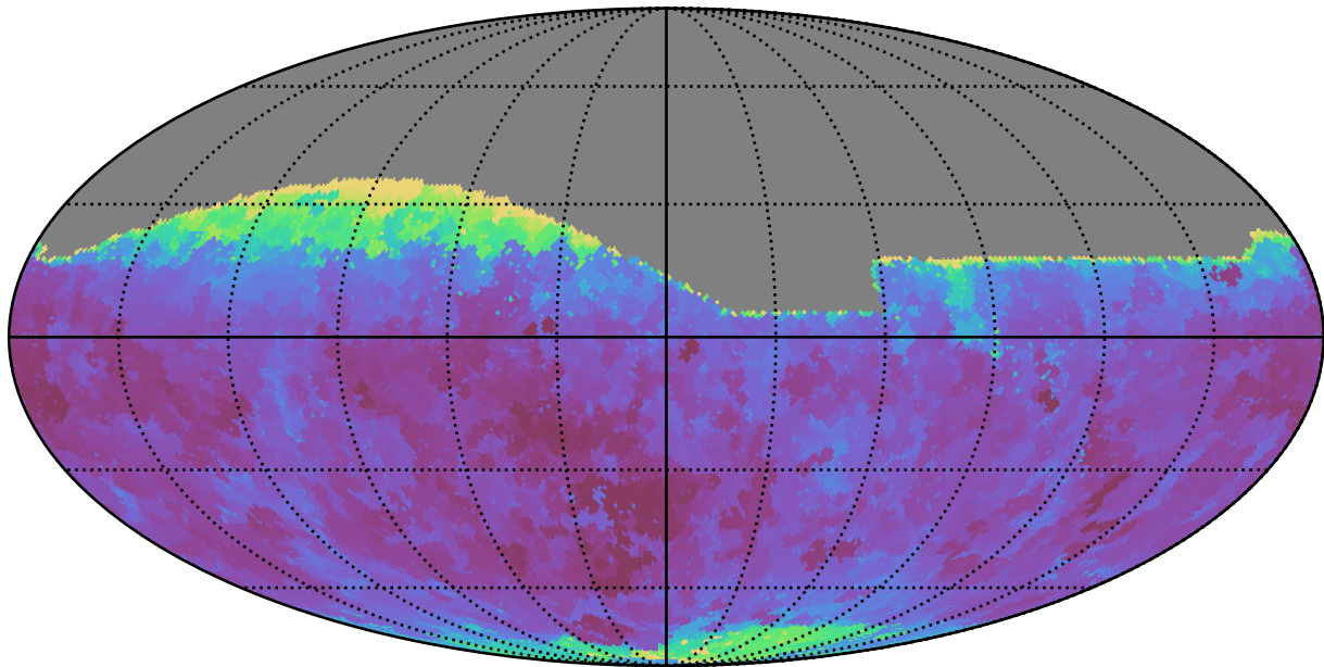
too_elab_r8_d2_griz_v3.4_10yrs All sky g band: Min seeingEff
