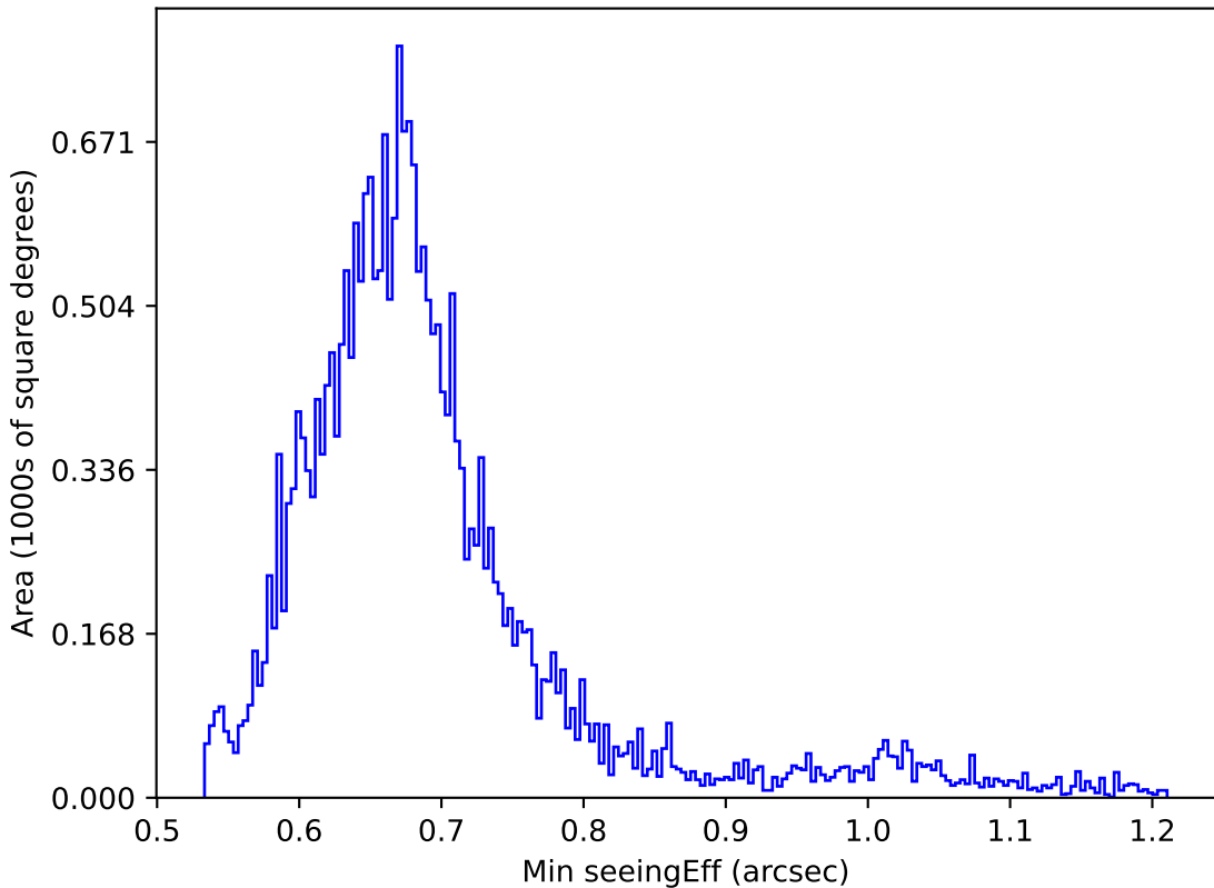
too_elab_r8_d2_griz_v3.4_10yrs All sky g band: Min seeingEff
