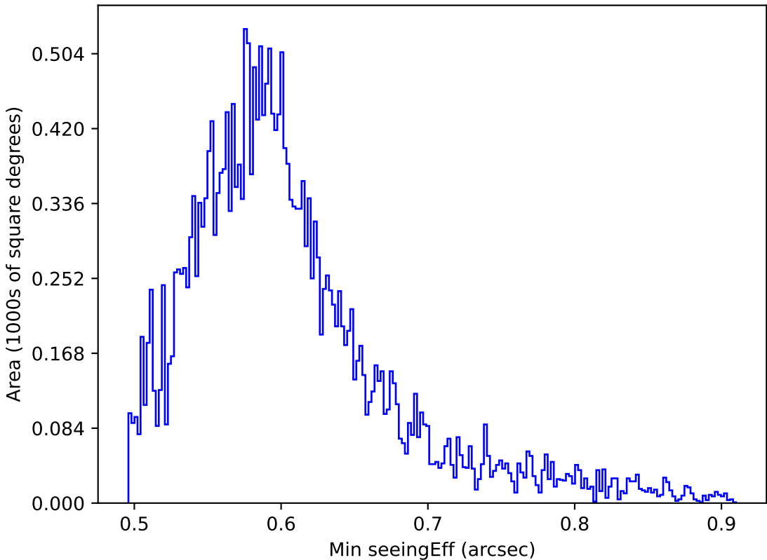
too_elab_r8_d2_griz_v3.4_10yrs All sky all bands: Min seeingEff
