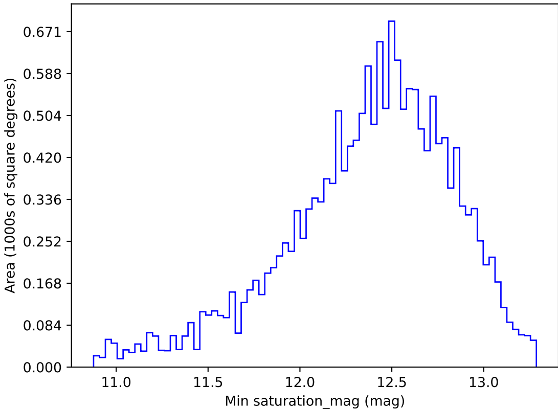
too_elab_r8_d2_griz_v3.4_10yrs WFD i band: Min saturation_mag
