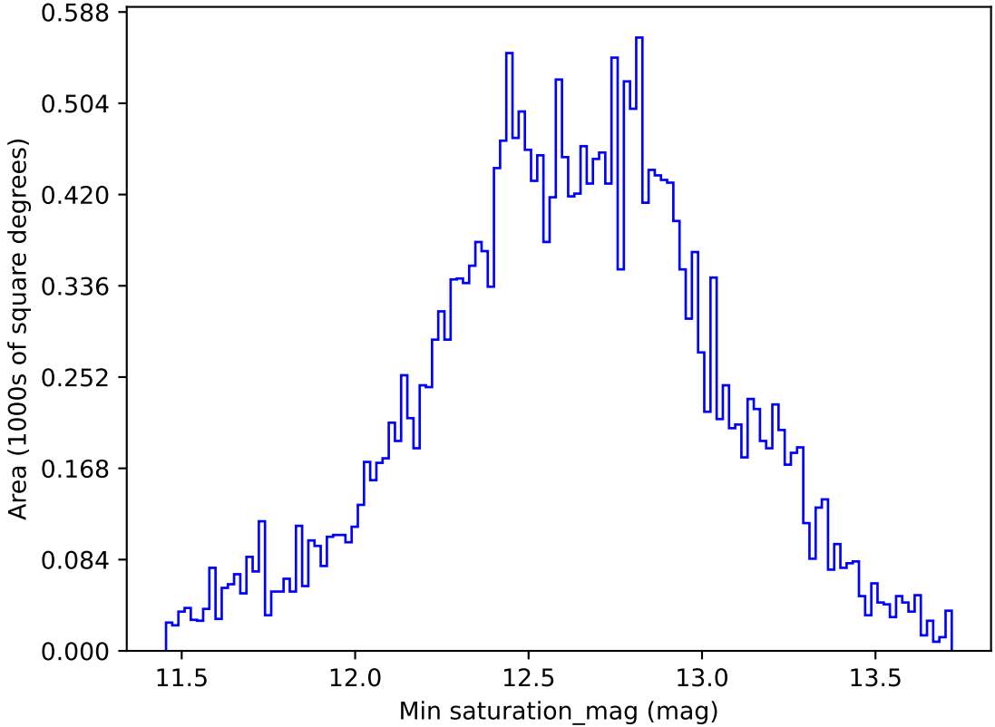
too_elab_r8_d2_griz_v3.4_10yrs All sky r band: Min saturation_mag
